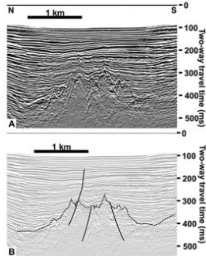
Figure 5. a) Uninterpreted and (b) interpreted profile extending across the central part of the lake from north to south. The crestal graben is not observed on this profile. Note several normal faults that extend up into the sediment section. The uppermost ~40 ms (TWTT) of sediment section contains distinctly lower amplitudes than the deeper sediment section reflections. This sequence is composed of high-water content lacustrine muds, sitting on top of a desiccation surface. The edge of the annular moat is observed on the margins of this profile. Modified from Scholz et al. (2007).
