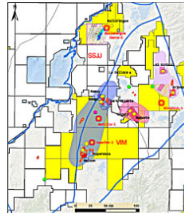
Figure 5. New discoveries by the companies Canacol Energy and Lewis Energy-Hocol, are located outside the ANH 2022 prospective corridors, for the Sinú San Jacinto SSJJ and lower Magdalena Valley VIM basins.
