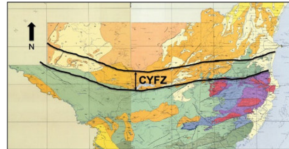
Figure 5. Geological map of Belize and northern Guatemala. The Central Yucatan Fault Zone (CYFZ) separates Paleozoic/Mesozoic rocks (blue, red and green) south of the fault zone from Tertiary rocks (earth tones) exposed within and north of the fault zone. Map from Bonis, Dengo and Bohnenberger, 1960.
